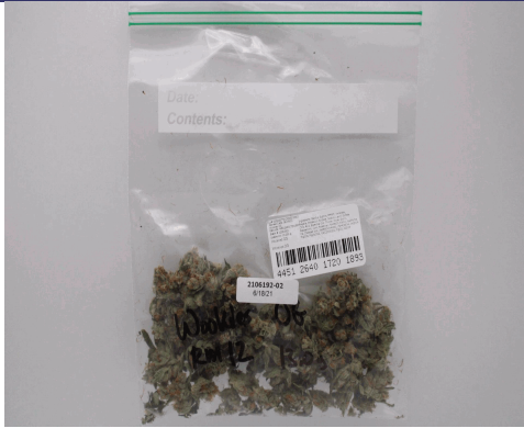
Cannabinoid (HPLC) Analyzed: 06/29/21 By: CBH
